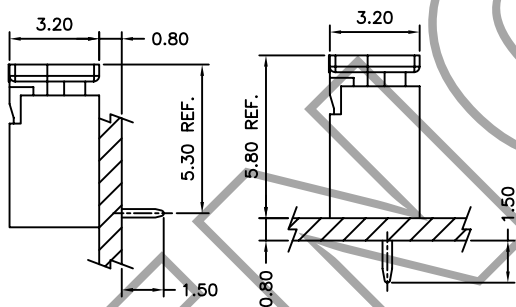
DIP TYPE
